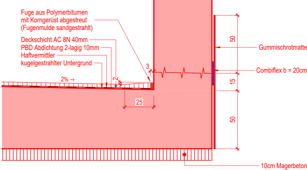
Detail Boden - Wand, 1:20
