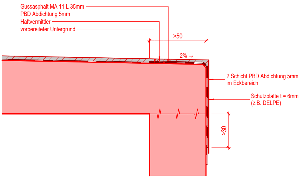
Detail Wand - Decke, 1:20
